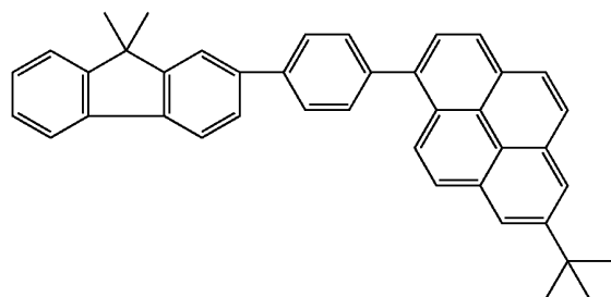
Compound 16
