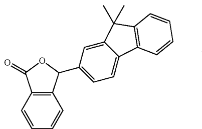
Compound 22
