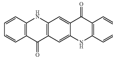
Quinacridone
