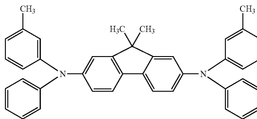
DTDPFL
