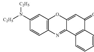
Nile red
