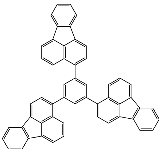
Compound 21
